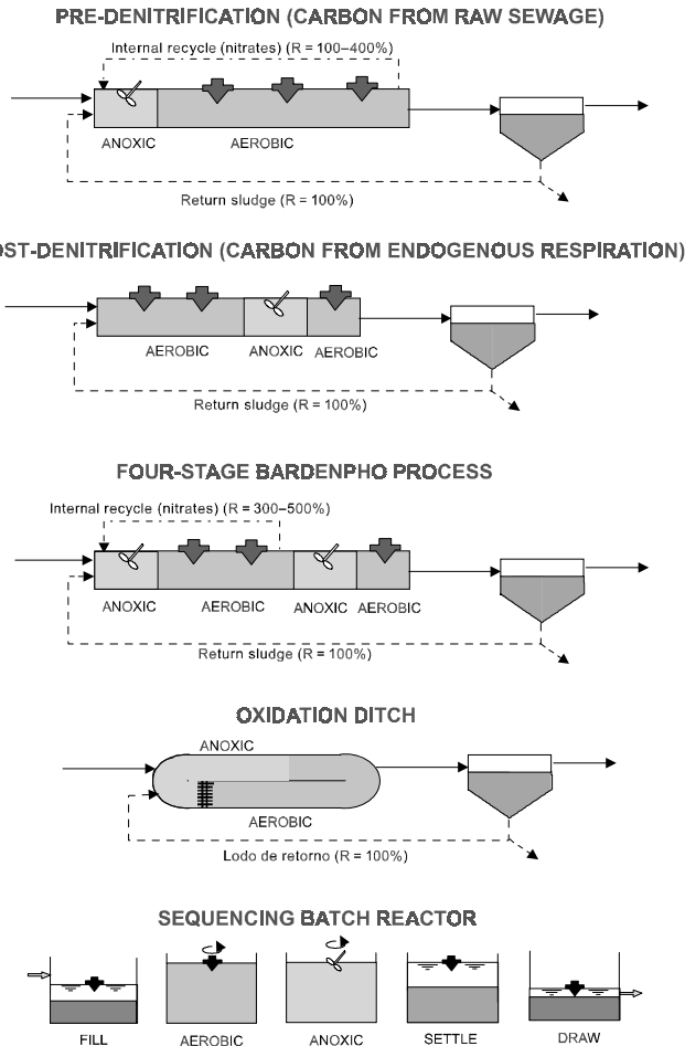
Figure 7.1. Main processes for biological nitrogen removal
